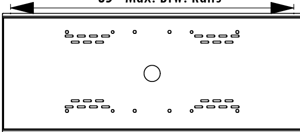
FSUL3520 Mounting Plate 35" Max. Btw. Rails
