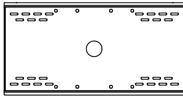
FSUL2014 Mounting Plate 20" Max. Btw. Rails
