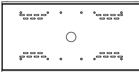
FSUL2720 Mounting Plate 27" Max. Btw. Rails
